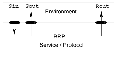
Fig. 6. SPIN’s validation model of the BRP and FTS.
